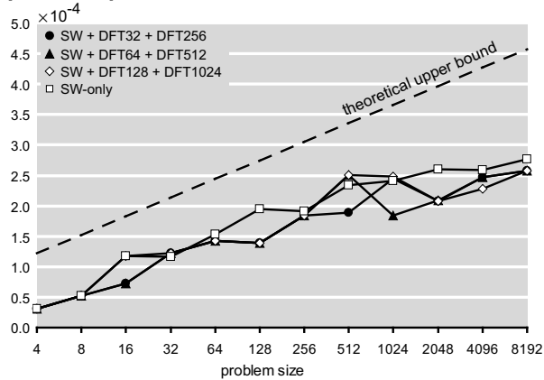
(a) DFT Maximum Error [absolute error]
