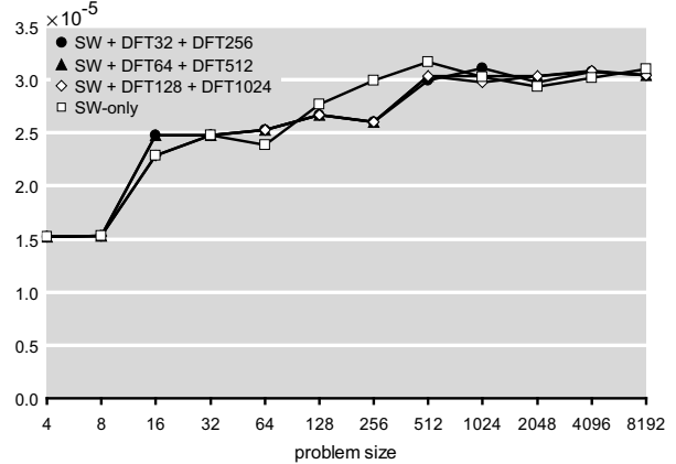
(b) DFT Average Error [absolute error]
